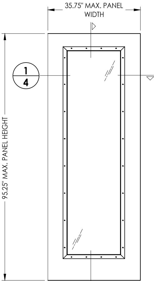
2 4 SIDELITE PANEL JELD-WEN Steel (Wood Edge)
