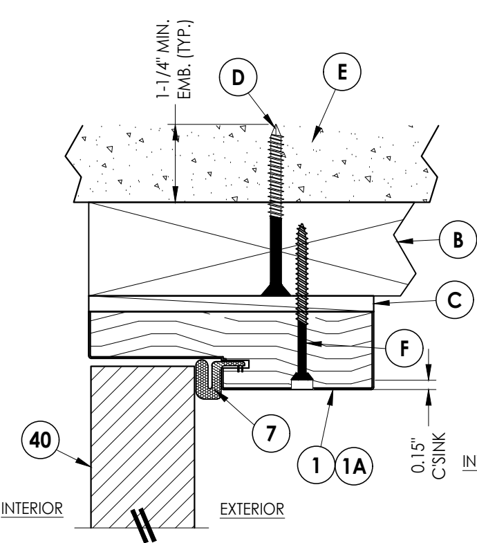
1 6 VERTICAL CROSS SECTION Inswing shown (Outswing similar) 2X Buck Construction
